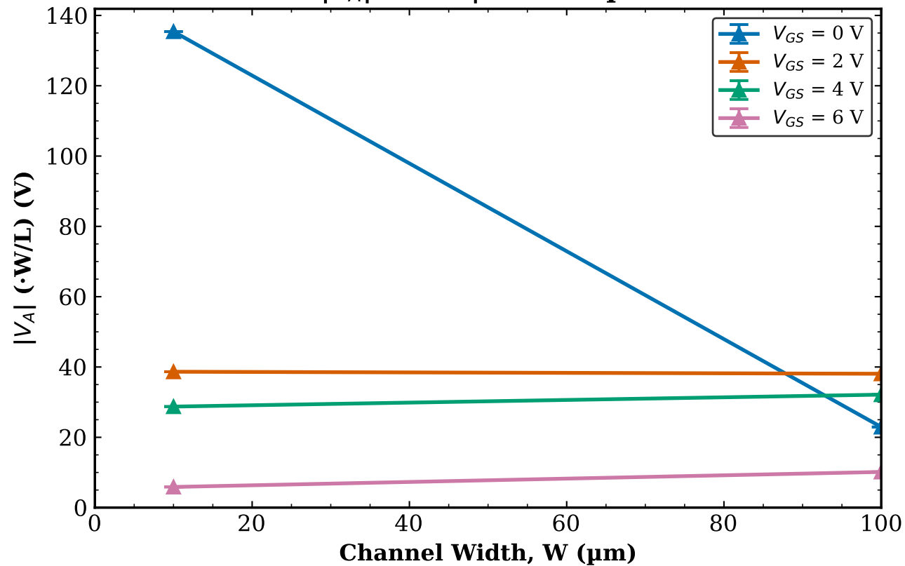
TFT3 Transistor 1 |V_A| vs W | L = 10\text{ }\mu\text{m}
